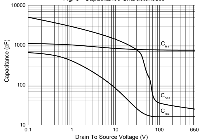
Fig. 6 - Capacitance Characteristics
