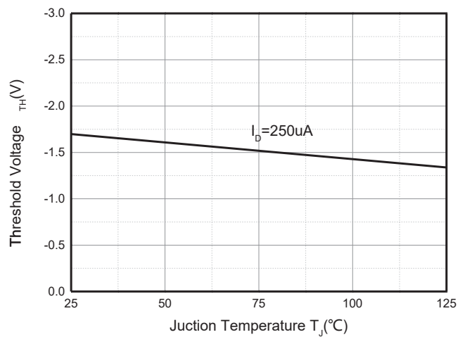
Threshold Voltage
